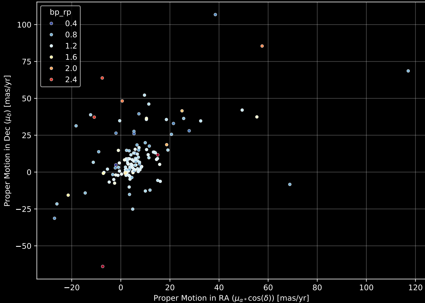
APOGEE DR17 Field: [LMC1] Proper Motion Diagram (n= 200)
