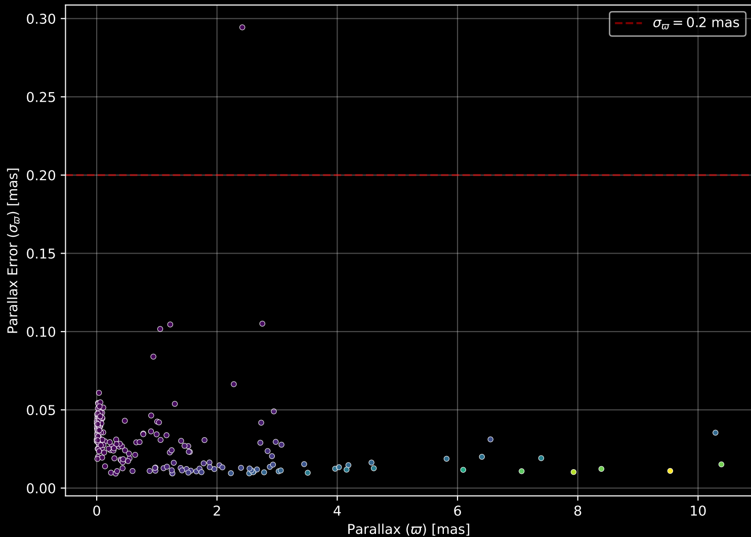
APOGEE DR17 Field: [LMC1] Parallax Quality (n= 200)
