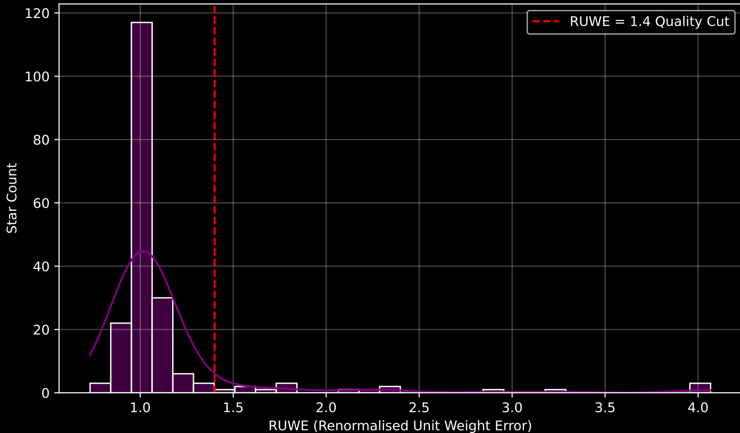
GAPOGEE DR17 Field [LMC1] RUWE Distribution (n= 197)
