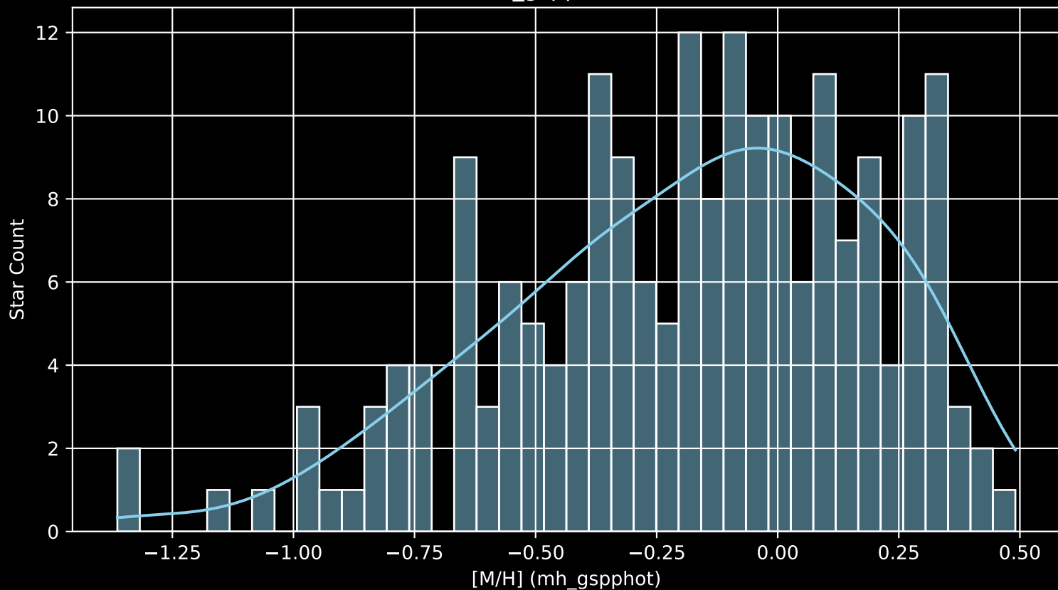
APOGEE DR17 Field: [LMC1 [M/H] (mh_gspphot) (n= 200)
