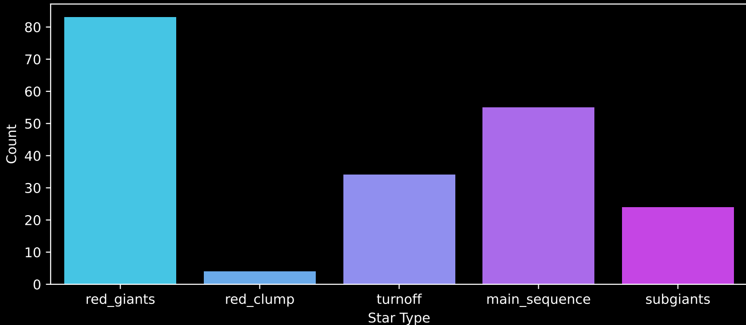
APOGEE DR17 Field: [LMC1] Count plot of Star Type
